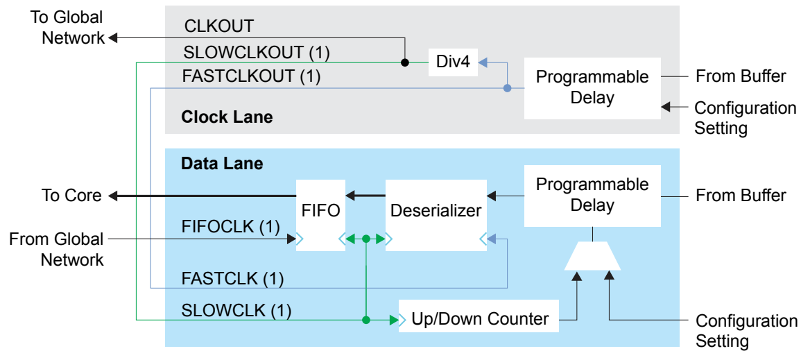
Figure 30: Connections for Clock and RX Data Lane in the Same MIPI RX Channel
