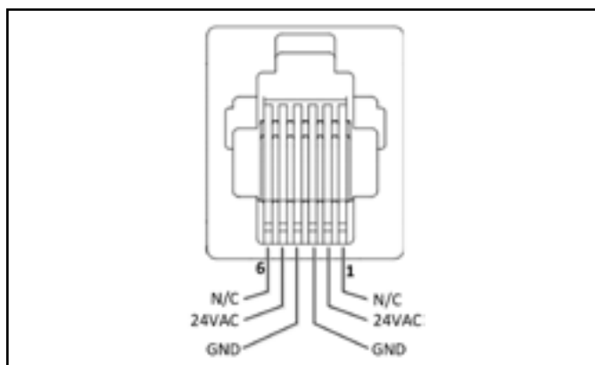
Figure 9. Pin-out of the console's power socket
