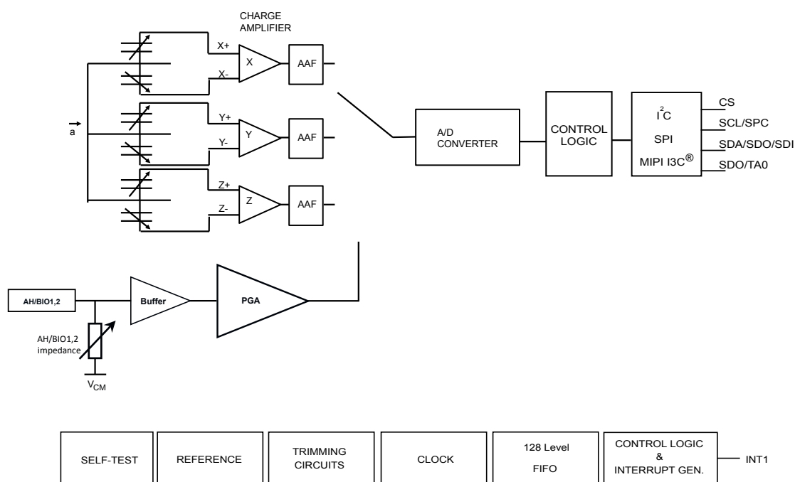
Figure 1. Block diagram
