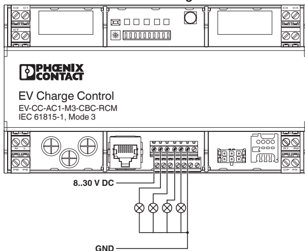
Connection diagram
