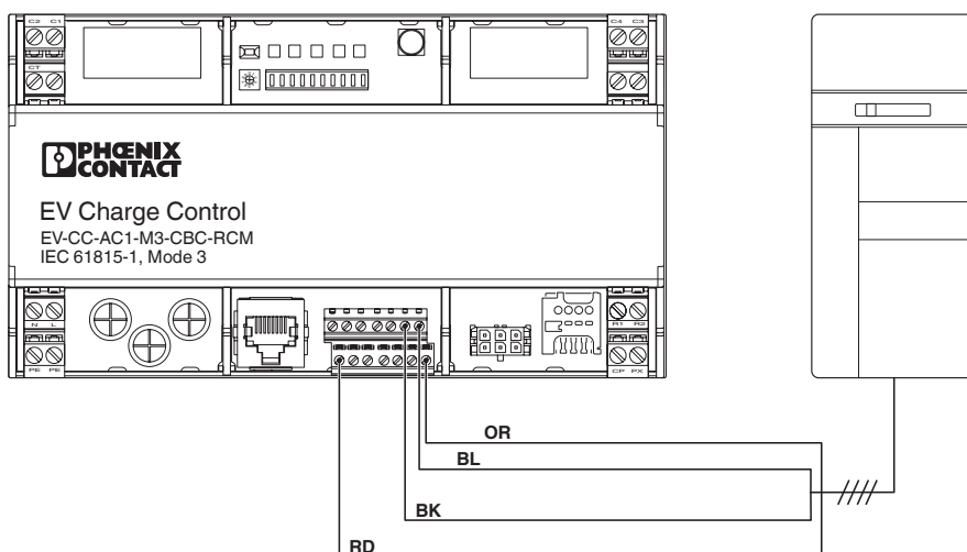
Connection diagram
