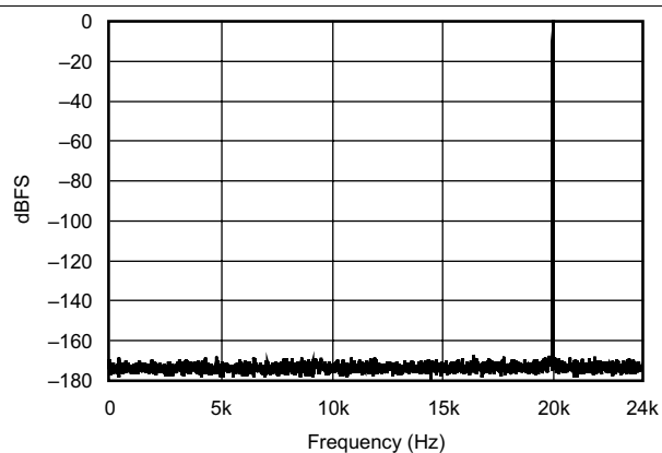
Figure 35. FFT With 20-kHz Input Tone at 0 dBFS
