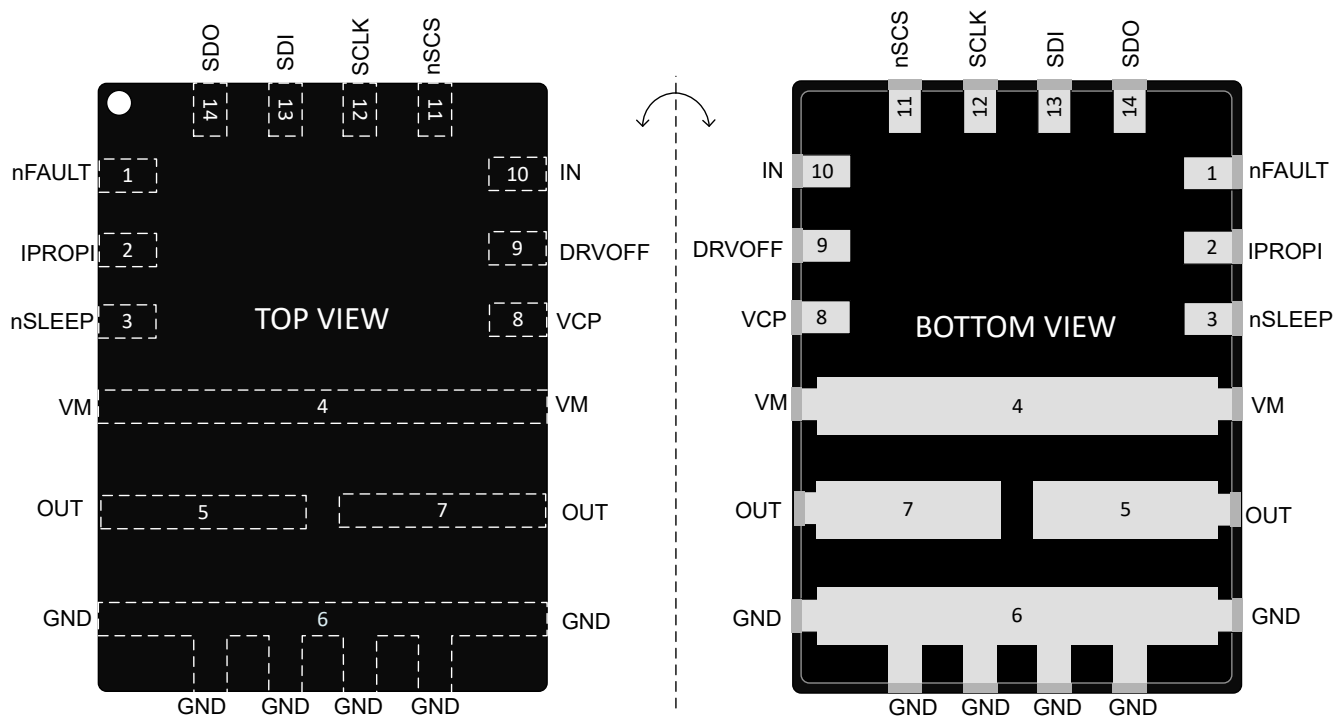
Figure 5-4. DRV8143S-Q1 SPI(S) variant in VQFN-HR (14) package
