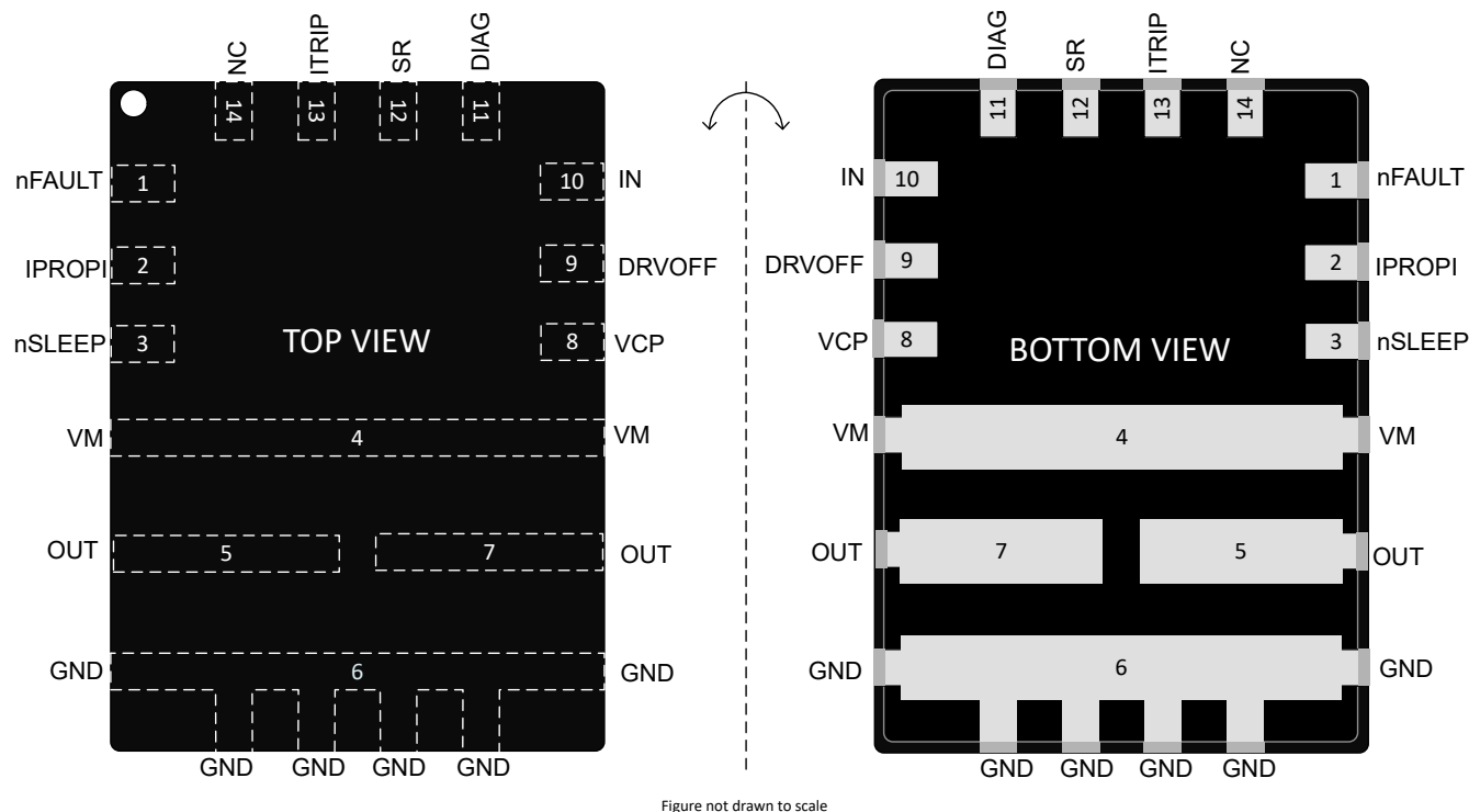
Figure 5-1. DRV8143H-Q1 HW variant in VQFN-HR (14) package
