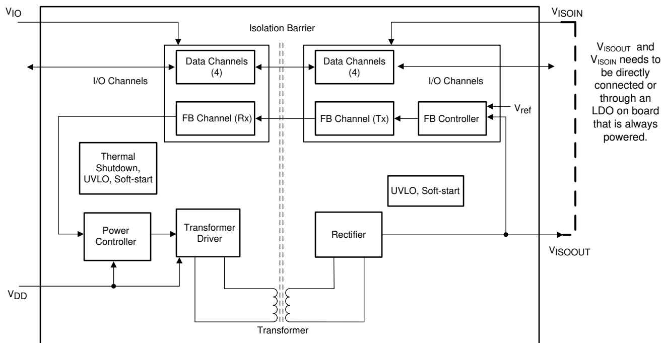
Figure 9-1. Block Diagram
