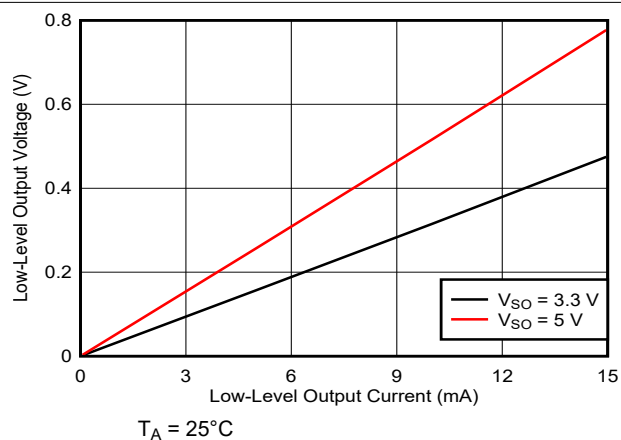
Figure 7-18. Low-Level Output Voltage vs Low-Level Output Current
