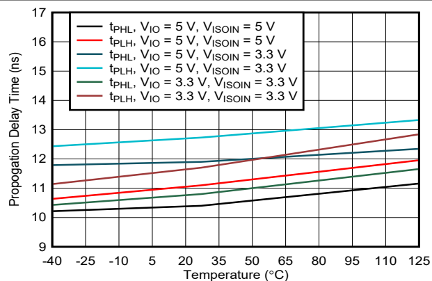
Figure 7-16. Propagation Delay Time vs Free-Air Temperature
