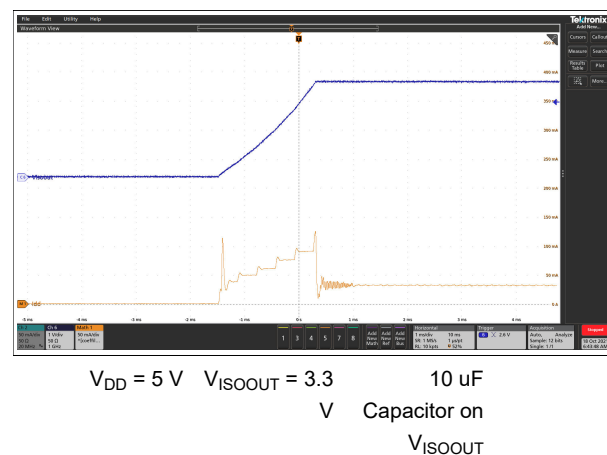
Figure 7-20. Soft Start at 10-mA Load For V_{ISOOUT} = 3.3V
