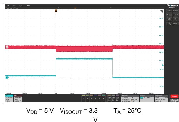
Figure 7-19. 10-mA to 110-mA Load Transient Response
