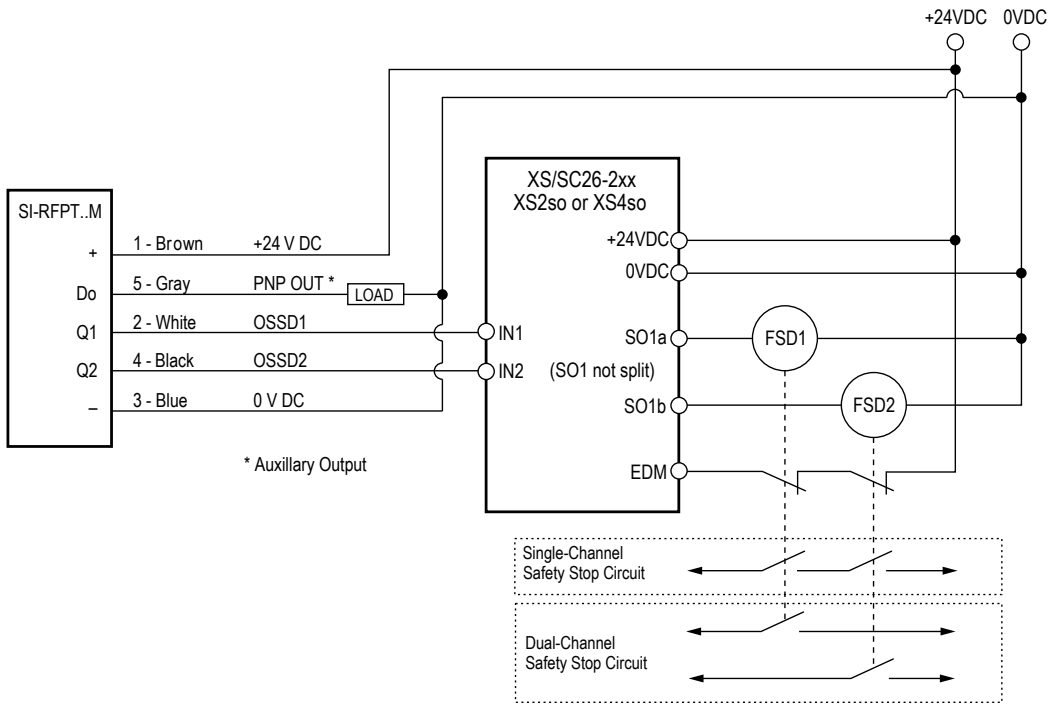
Wiring for a single PNP
