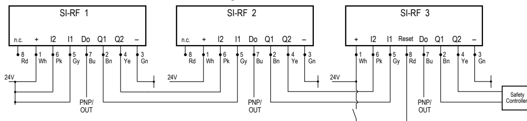
Wiring the switch in series
