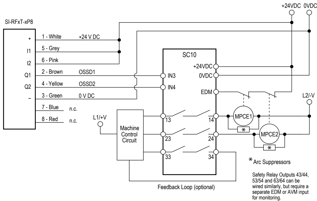
Wiring for a single 8-conductor sensor
