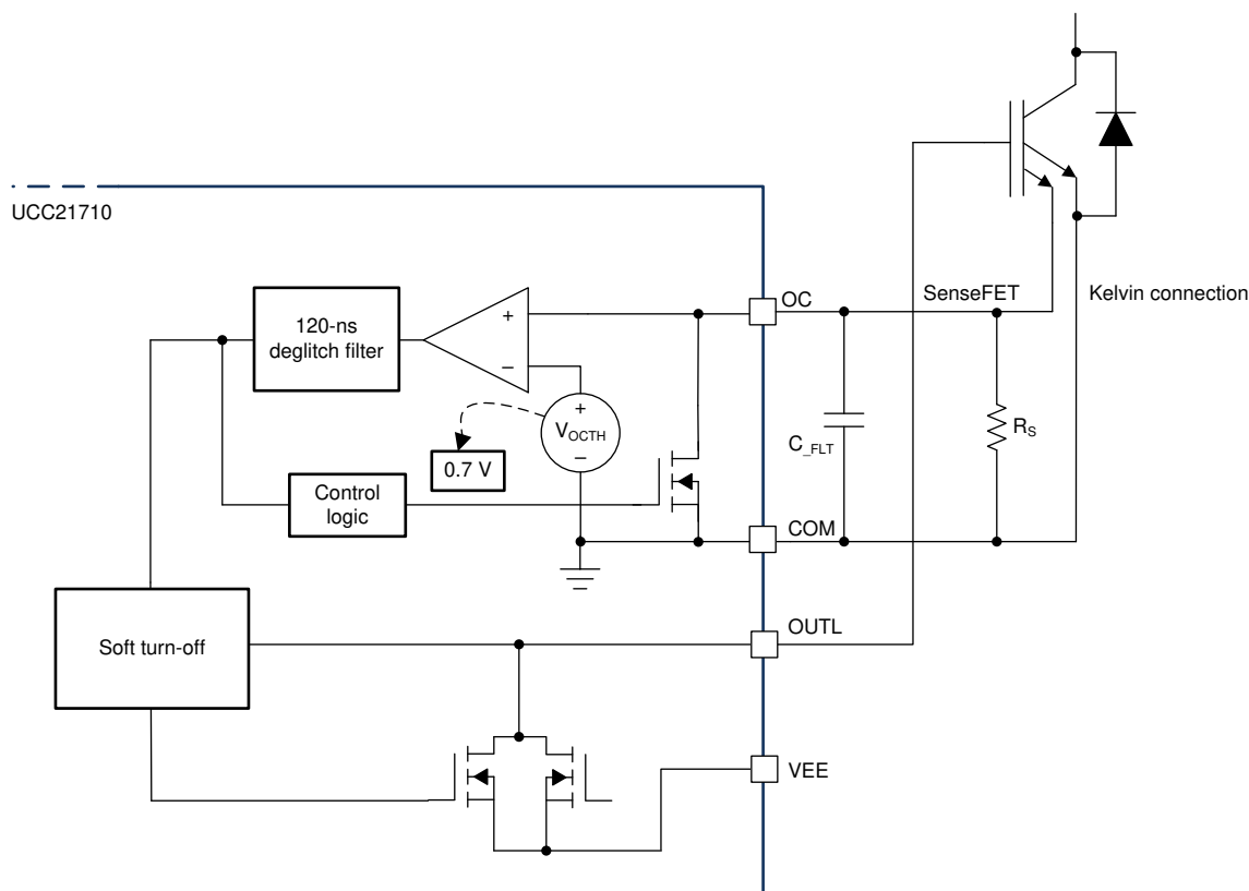
Figure 7-6. Soft Turn-Off
