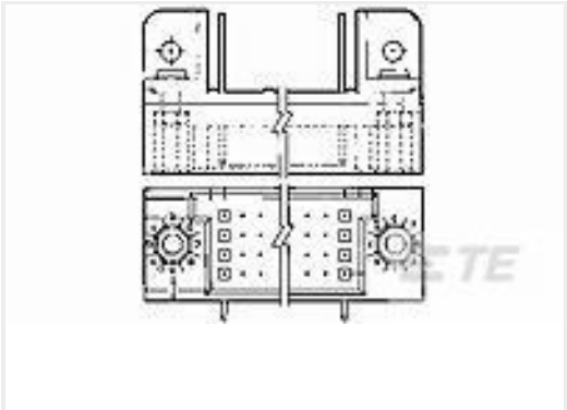
TE Part #533286-9 HDI PIN ASSY 4 ROW 240 POS R/A
