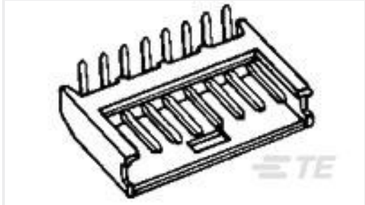
TE Part #280382-1 15P MODU II SHRD HDR, RT ANG, TIN
