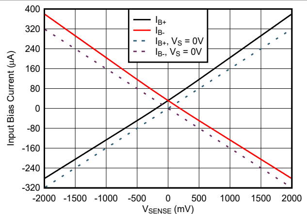
Figure 6-18. INA241x1 Input Bias Current vs V_{\text{SENSE}}
