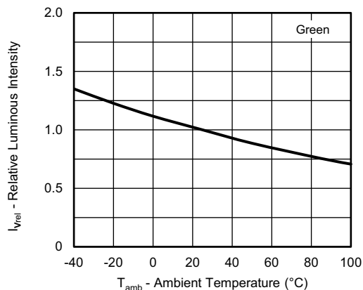
Fig. 21 - Relative Luminous Intensity vs. Ambient Temperature
