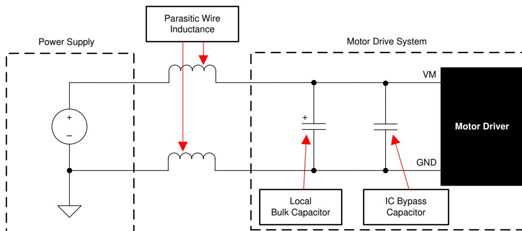
Figure 10-1. Motor Drive Supply Parasitics Example
