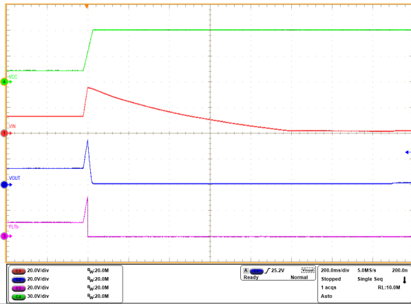
Figure 8-6. Overvoltage Response with External PFET for IN Voltage from 12 V to 60 V
