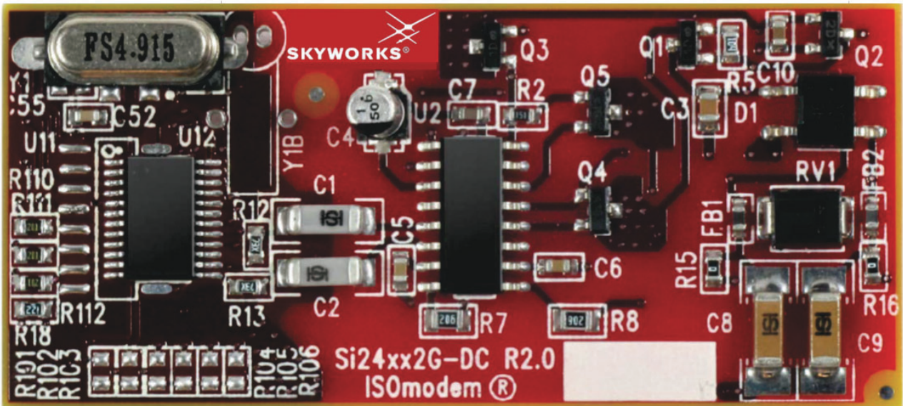
Figure 3. Daughter Card
