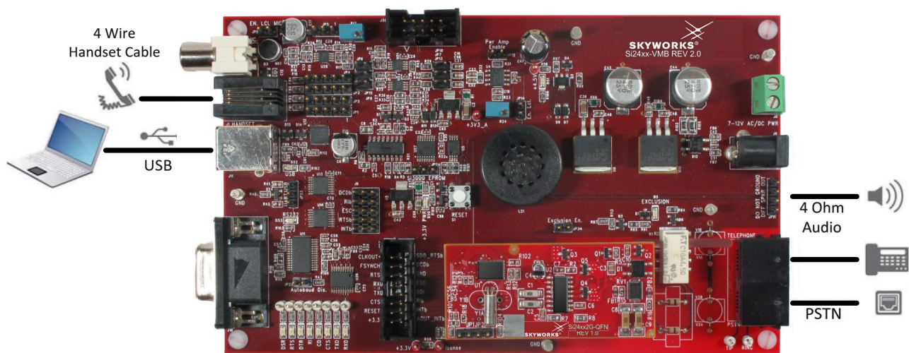
Figure 4. Global Voice ISOModem EVB Connection
