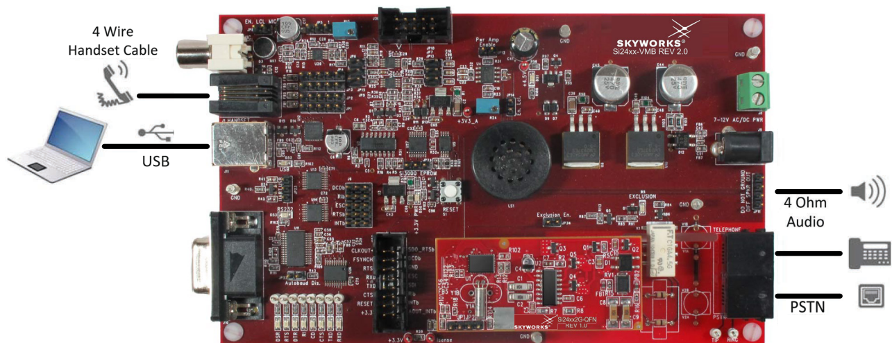
Figure 11. Sound Demonstration Hardware Interconnect Guide
