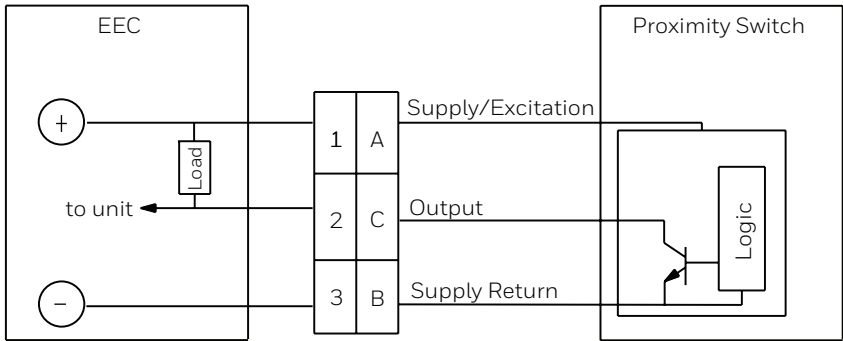
FIGURE 7. GAPS SERIES EN2997Y10803MN CONNECTOR
