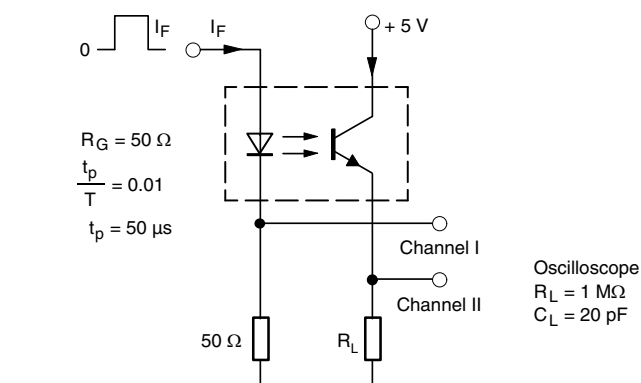
Fig. 2 - Test Circuit, Non-Saturated Operation
