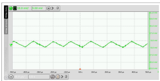
Figure 7-33. V_{ISOOUT} Ripple Voltage at 5 V with 10 \mu\text{F} Capacitor and 110 mA load
