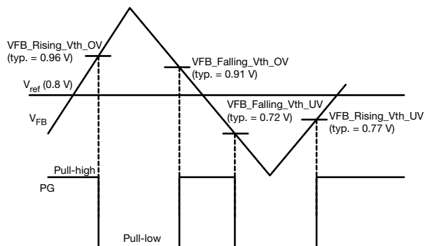
Fig. 9 - PGOOD Window
